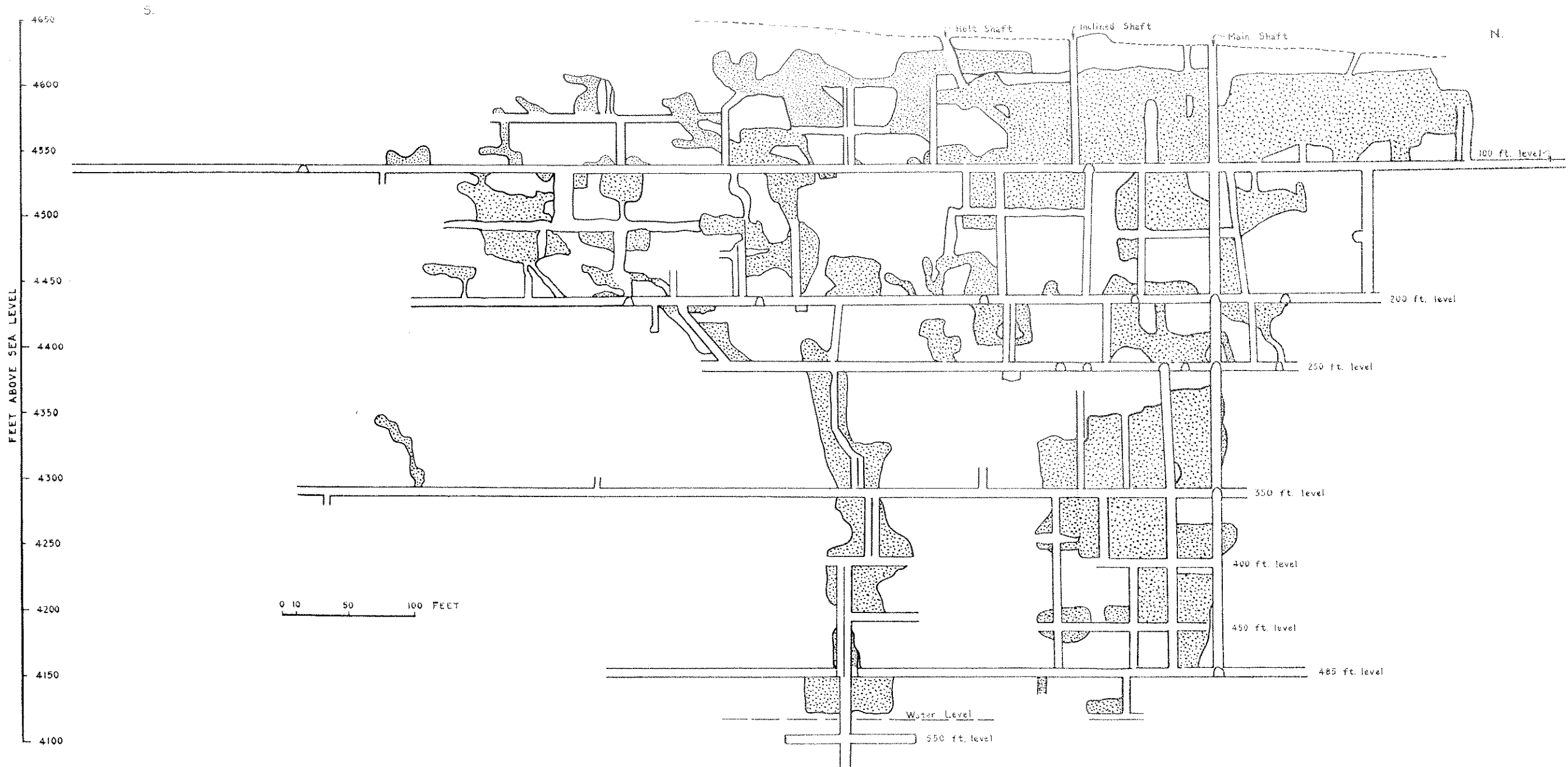
Plate X.—Longitudinal section of Tombstone Extension Mine, looking west. Stopes indicated by dotted areas.
