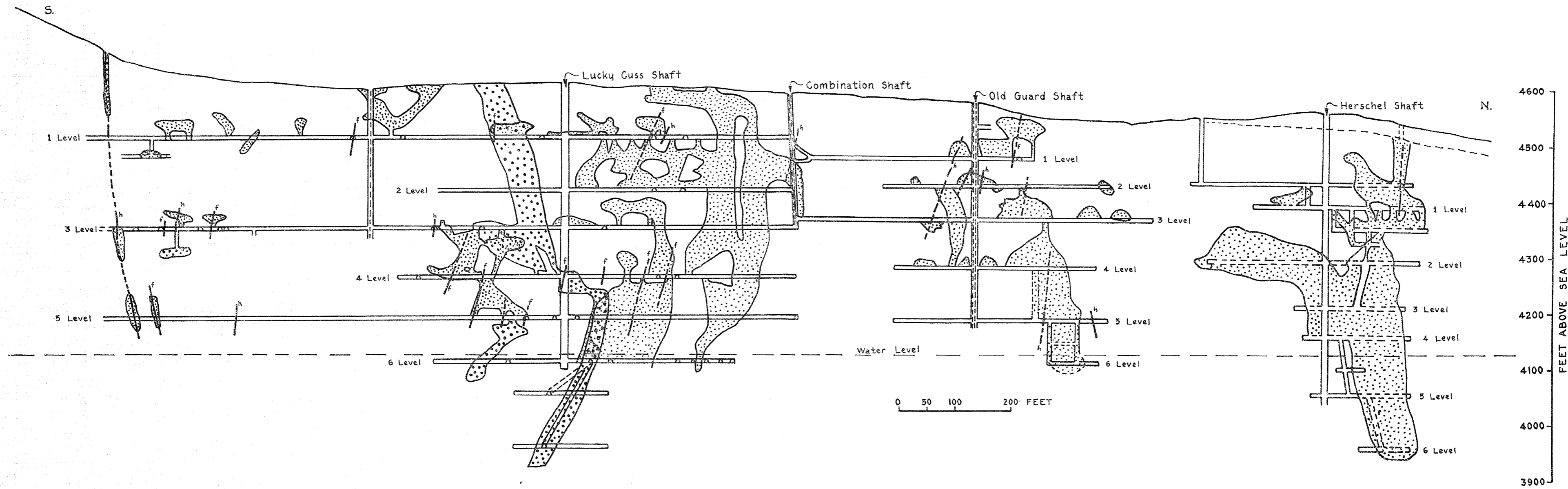
Plate XII.—Longitudinal section through Lucky Cuss, Old Guard, and Herschel mines, looking west. Stipes in Lucky Cuss fault zone indicated by small dots; stipes in massive limestone indicated by large dots; h , hanging-wall fissure; f , footwall fissure.
