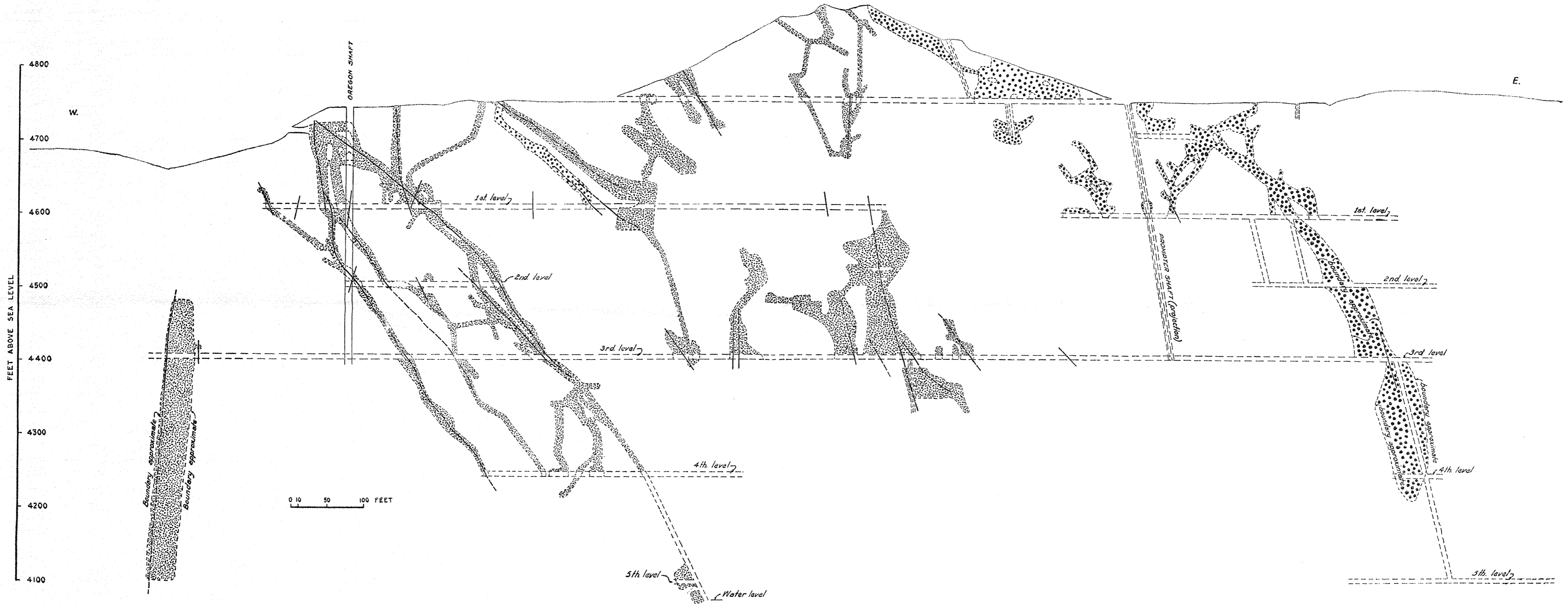
Plate XIV.—Longitudinal section through Oregon and Prompter mines, looking north. Stopes in Oregon slips indicated by small dots; stopes in Prompter fault indicated by large dots.
