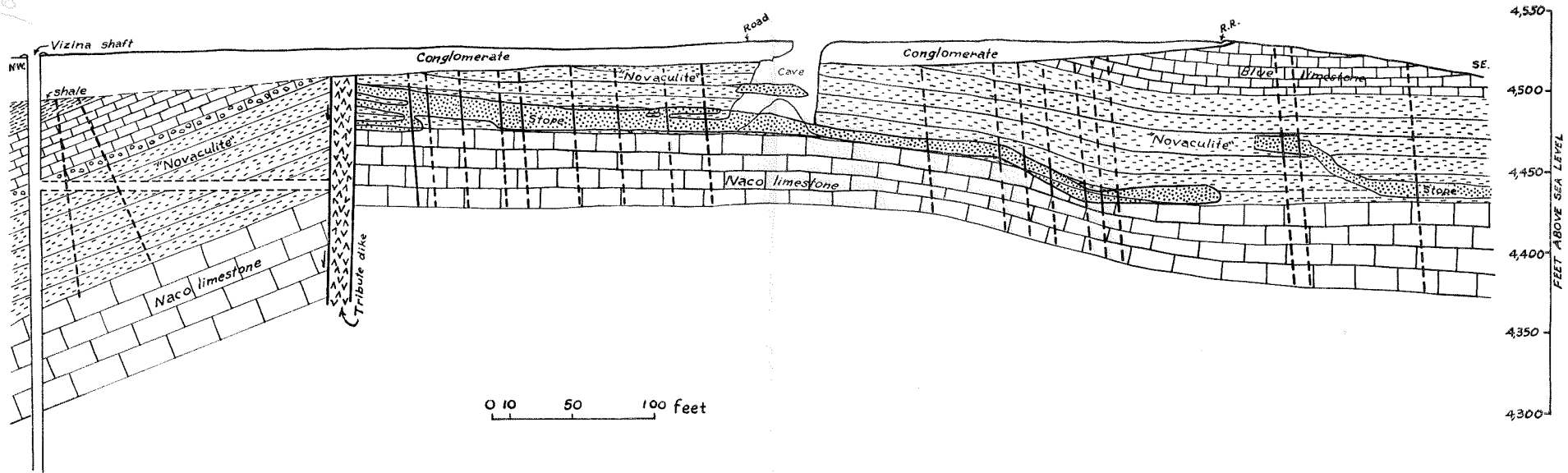
Plate XVIII.—Longitudinal section near axis of northeast Vizina roll, looking northeast.
