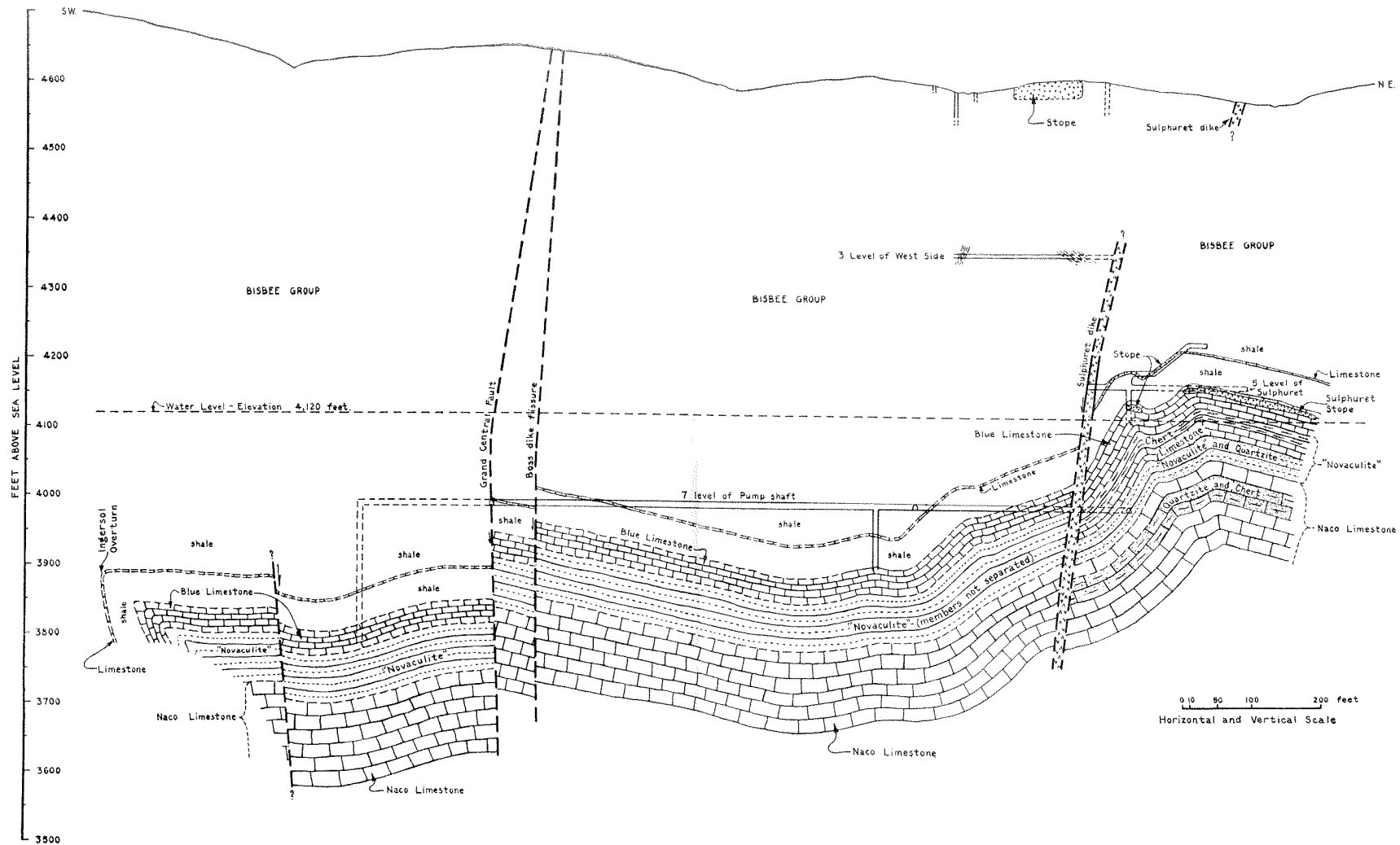
Plate XXII.—Section along Arizona Queen fissure, looking northwest.
