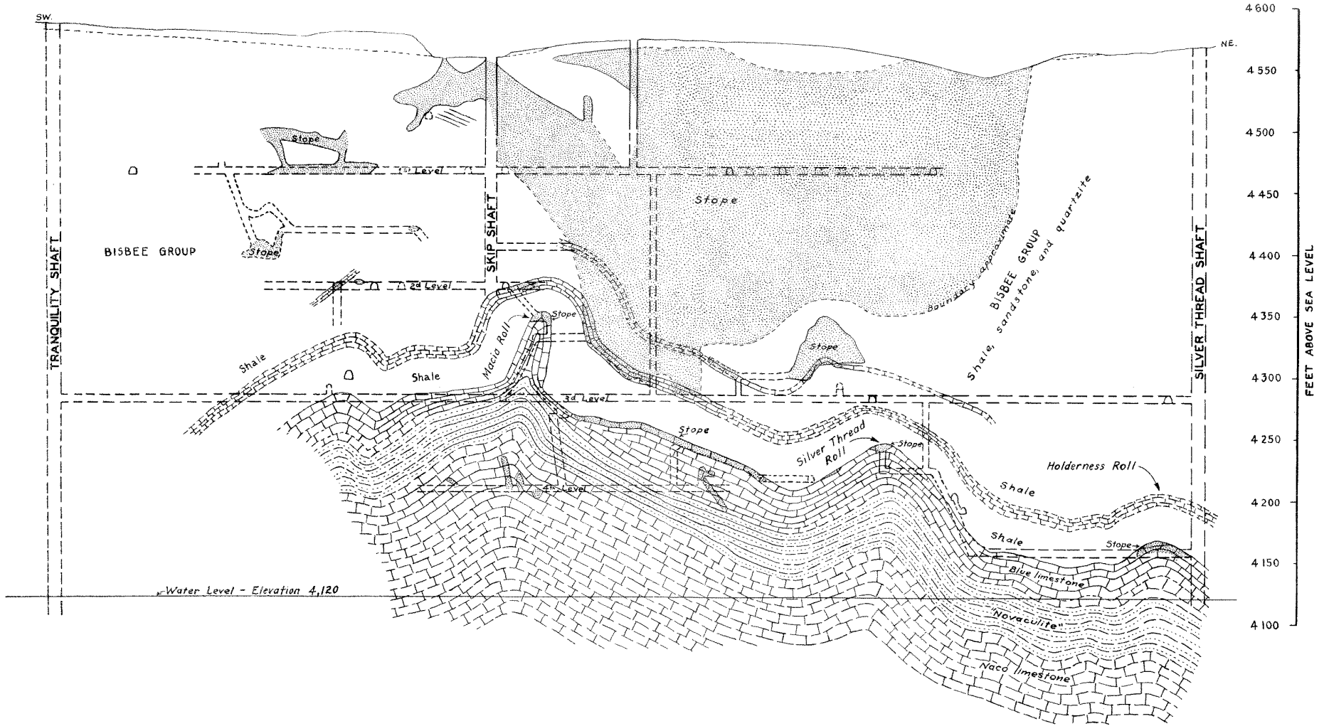
Plate XXIII.—Longitudinal section on Skip shaft fissure, looking northwest.
