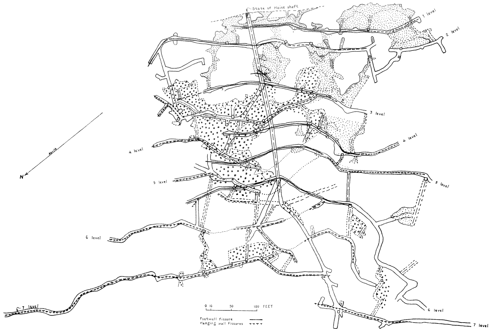
Plate XXV.—Plan of workings in State of Maine Mine, showing areas of stopping. Small dots indicate stopes in footwall fissure, large dots stopes in hanging wall fissures.
