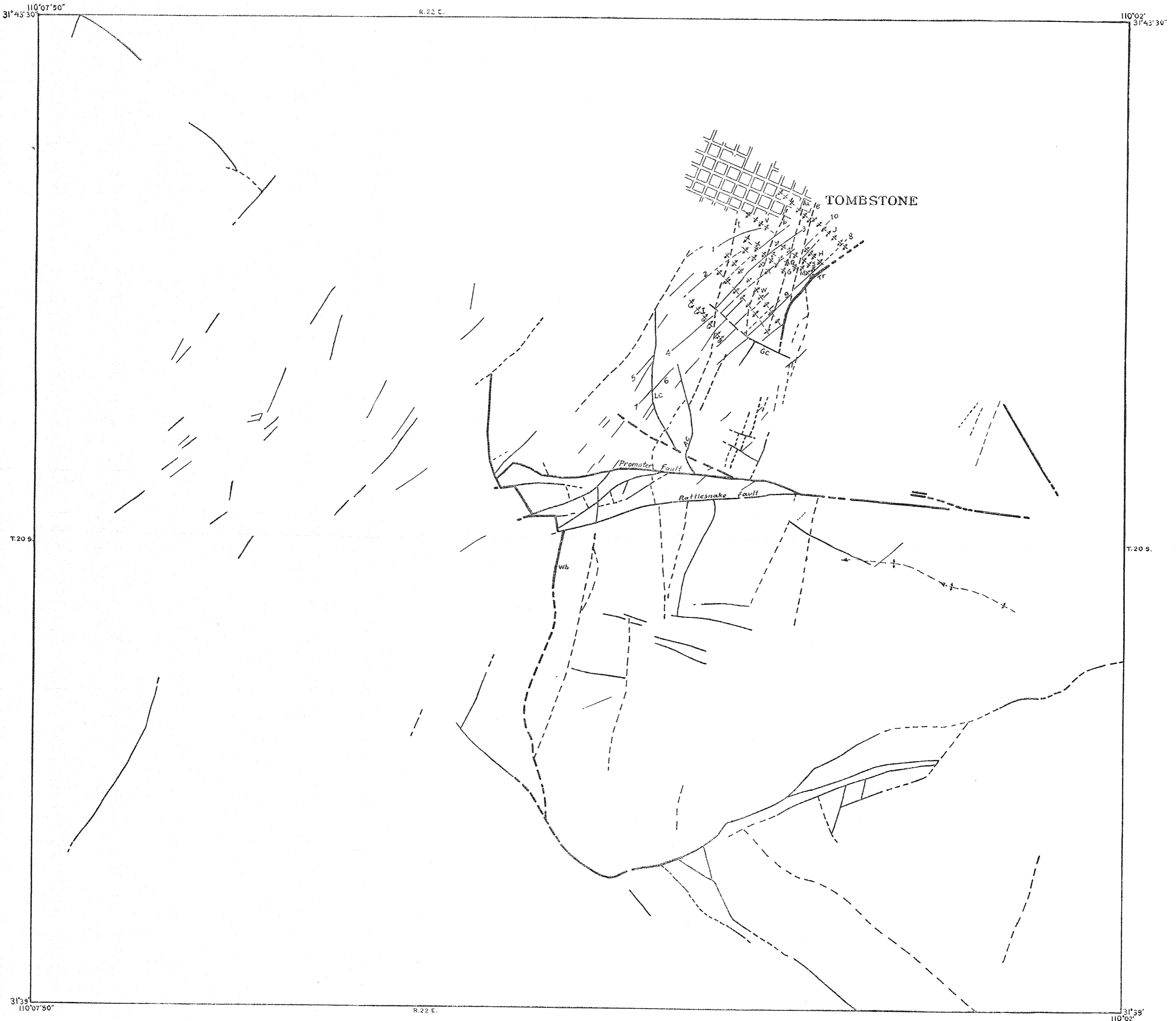
Plate VI.—Structure diagram of Tombstone district (place transparent paper over Plate III). I , Ingersol overturn; W , West Side roll; G , Girard roll; Q , Quarry roll; V , Vizina roll; S , Silver Thread roll; M , Macia roll; H , Holderness roll; J , Jeanes roll; t , Tribute dike fissure; b , Boss dike fissure; u , Sulphuret dike fissure; e , Empire dike fissure; Tr , Tranquility fault; GC , Grand Central fault; AC , Anchor or Coyote fault; LC , Lucky Cuss fault; Wb , west boundary fault; 1 , Defence fissure; 2 , Intervener fissure; 3 , West Side fissure; 4 , Blue Monday fissure; 5 , Rat shaft fissure; 6 , East Side fissure; 7 , Wedge fissure; 8 , Skip shaft fissure; 9 , Arizona Queen fissure; 10 , "409" fissure.
