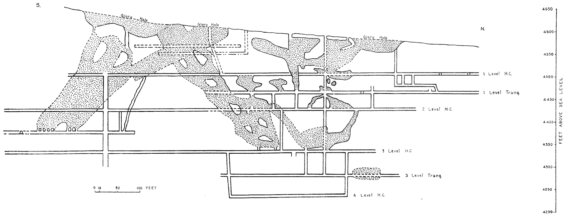
Plate IX.—Longitudinal section of workings in Head Center area, looking west. Stops indicated by dotted areas.
