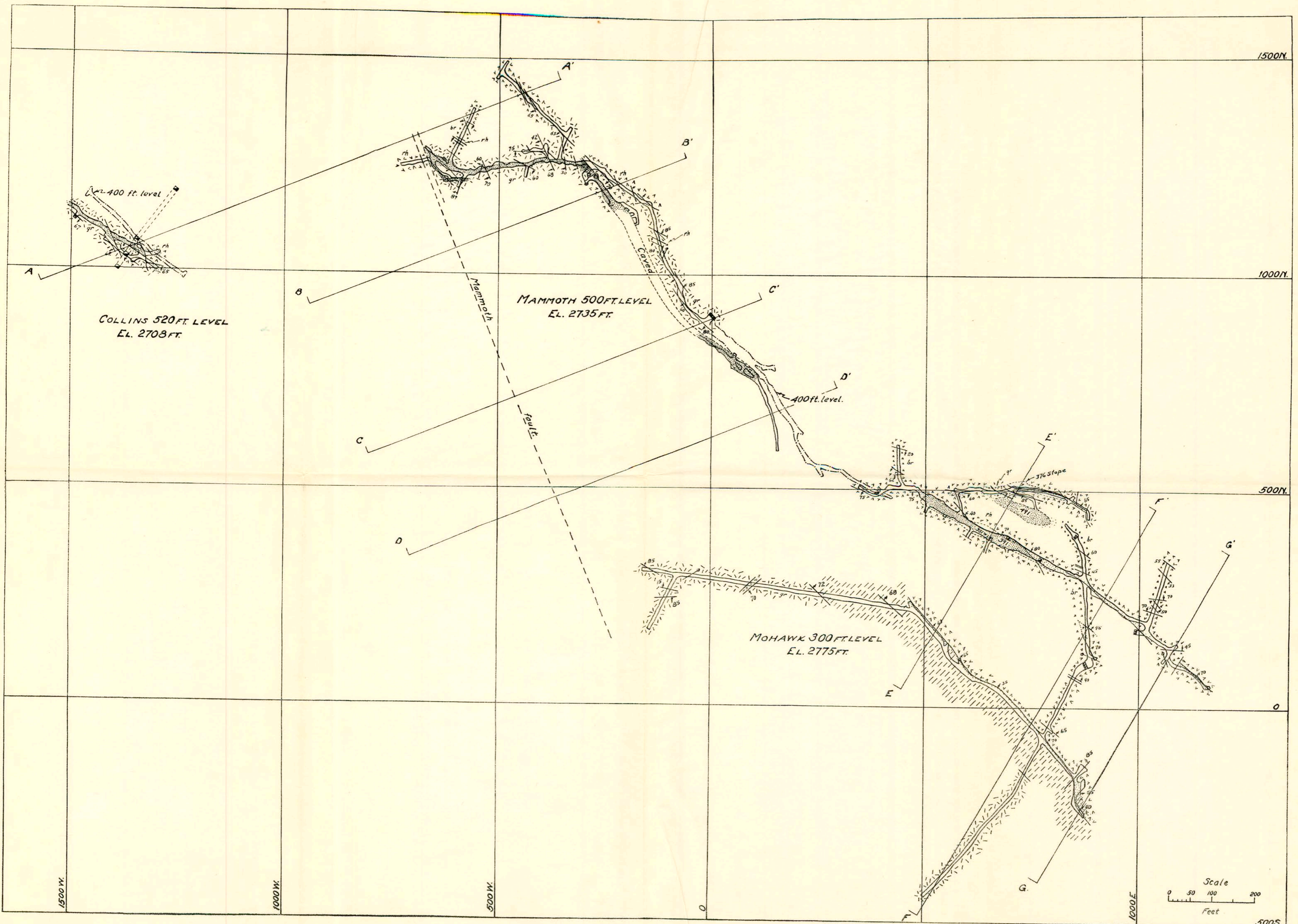
Plate VIII.—Geologic maps of Mohawk 300-, Mammoth 500-, and Collins 520-foot levels.
