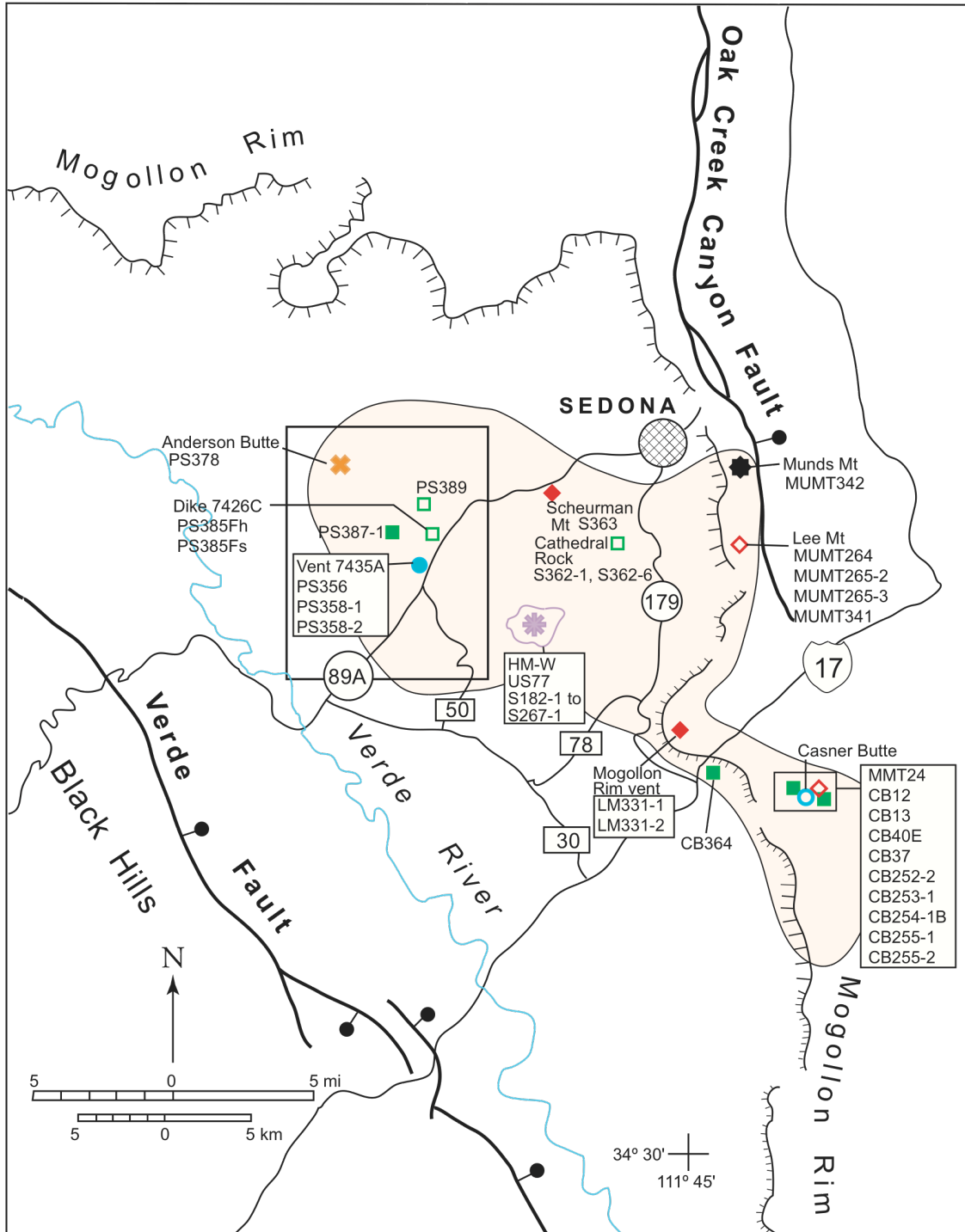
Appendix 1: Map Showing Locations of Analyzed Samples. Sample locations on the Page Springs Quadrangle (large box) are shown on Holm, 2015, Sheet 4; sample locations in the summit area of House Mountain (lavender asterisk with enclosure) are shown on Holm and Wittke, 1996, Sheet 1.
