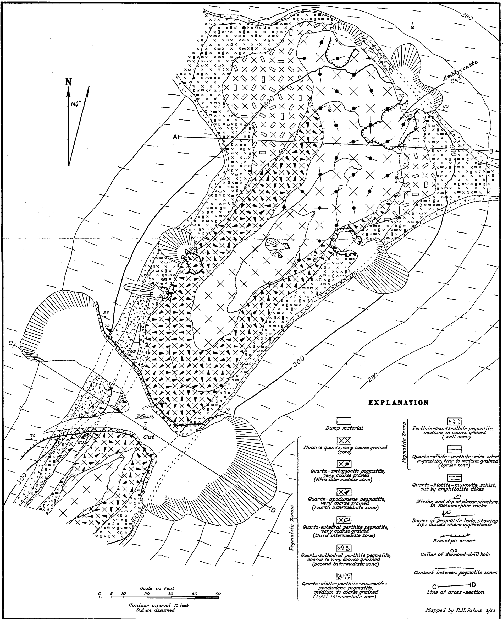
Plate XVII.—Geologic map of the North Morning Star mine.
