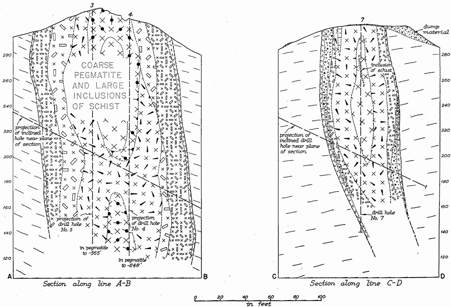
Plate XVIII.—Cross sections through the north pegmatite body, Morning Star mine, showing distribution of pegmatite zones as interpreted from exploratory drill holes. See Plate XVII for locations of sections and explanation of rock units.
